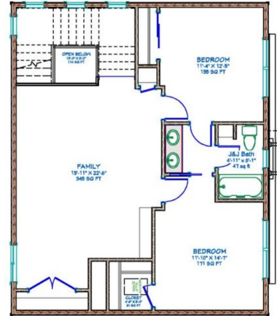
2nd Floor
