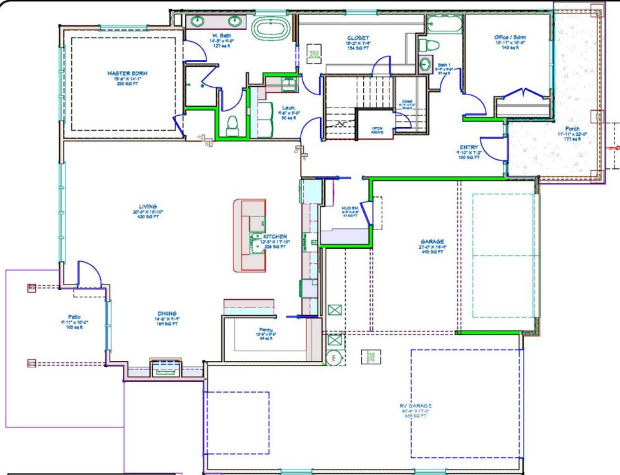
1st Floor
